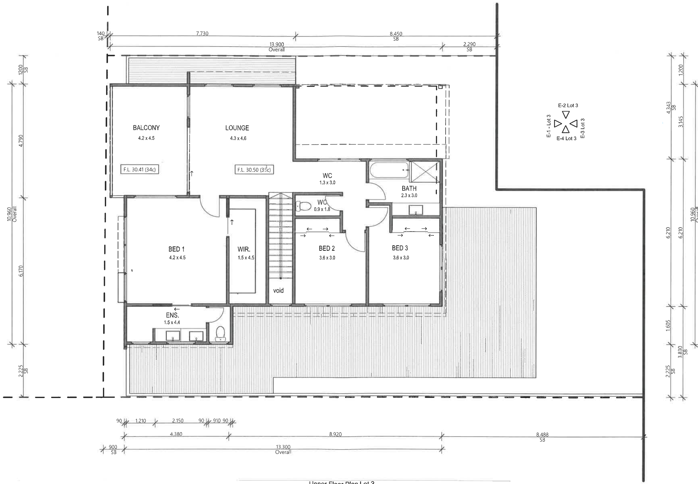
1. Upper Floor Plan Lot 3 1:100
